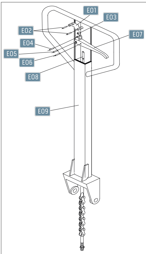
YOKE ASSY
